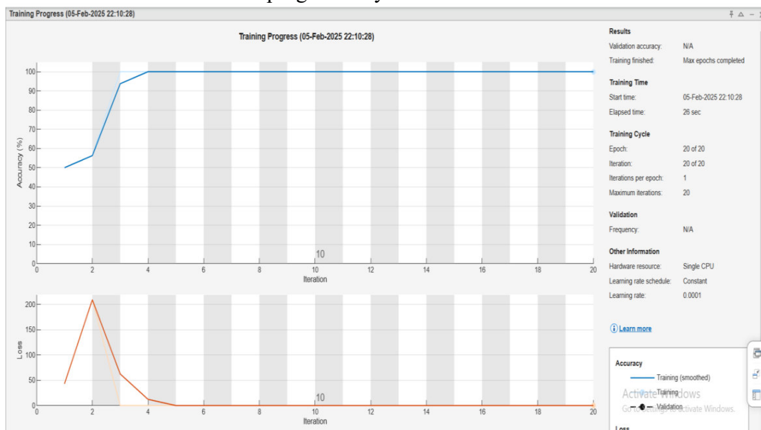
Fig.5. Training Progress
