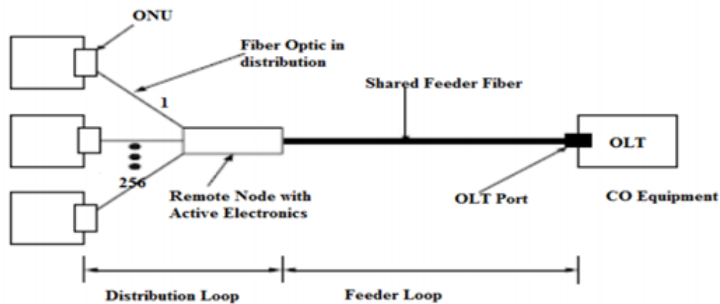
Figure (7) : Active Optical Network (AON)
