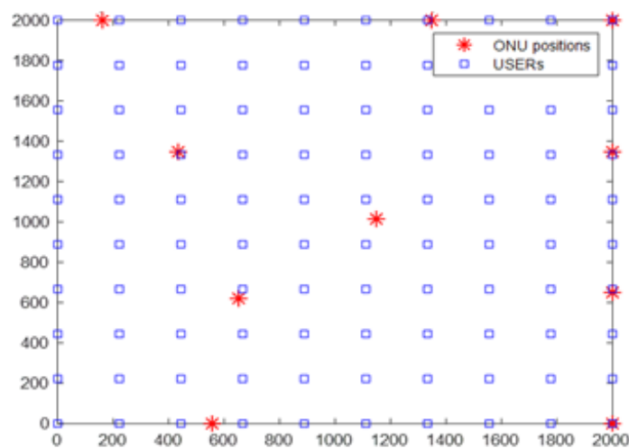
a - optimized antenna positions by using AOA algorithm
