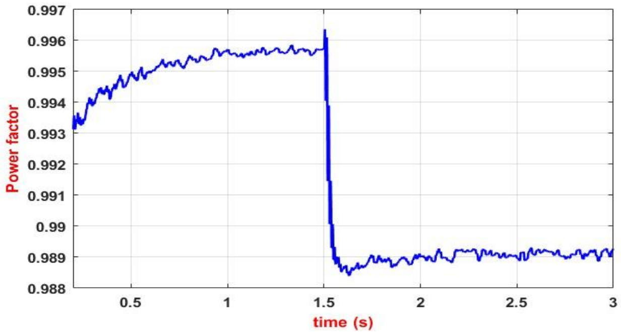
Figure 9. The power factor for each phase of the input side under PI-based control obtained from the Simulink simulation results.
