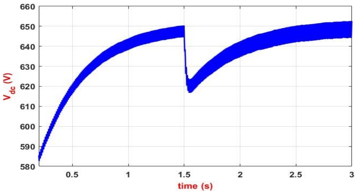
Figure 10. Total DC-link voltage response of the system obtained from the Simulink simulation under PI-based control.
