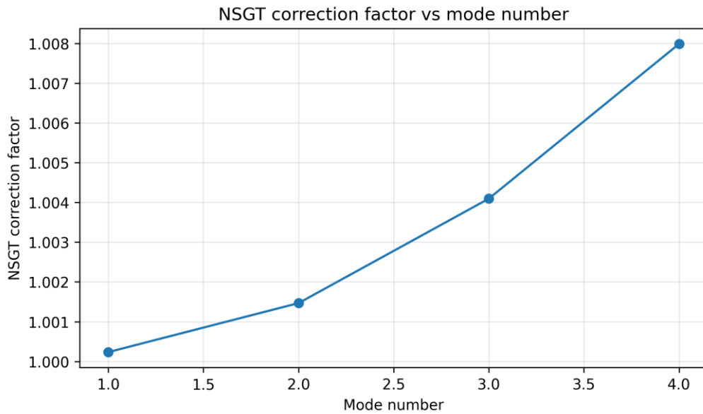
Fig. 18. NSGT correction factor for the first four modes in the reference nano-beam.
